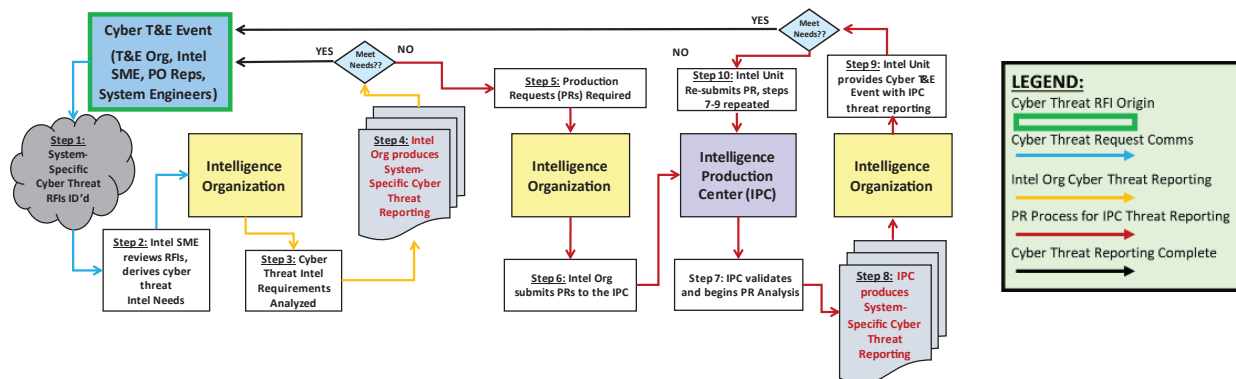
Figure D-2. Intelligence Unit and IPC Cyber Threat Production Flowchart
