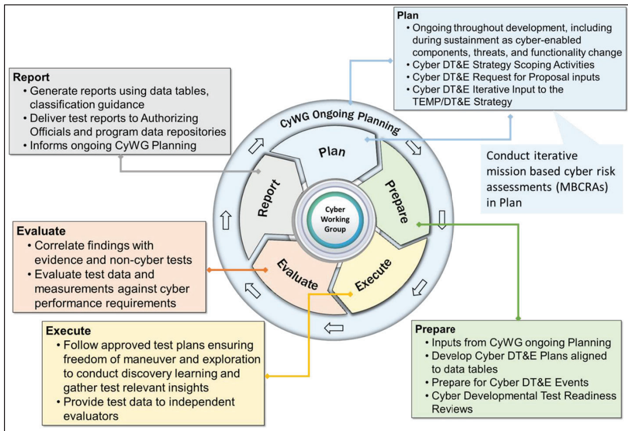
Figure 2-1. Cyber DT&E Iterative Process
