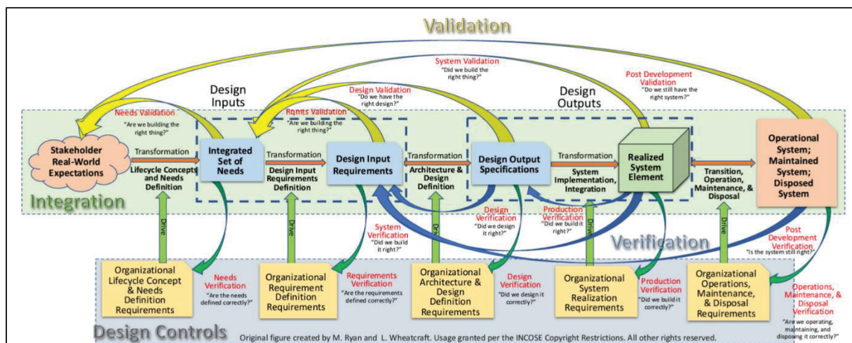
Figure B-4. Verification and Validation Occurs Throughout the Life Cycle
