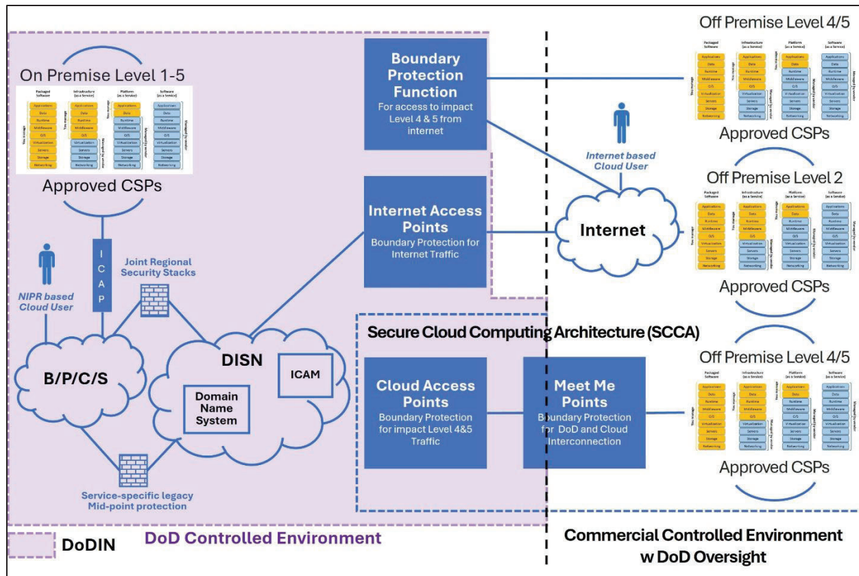
Figure H-3. Cloud Integration with the DoDIN Architecture
