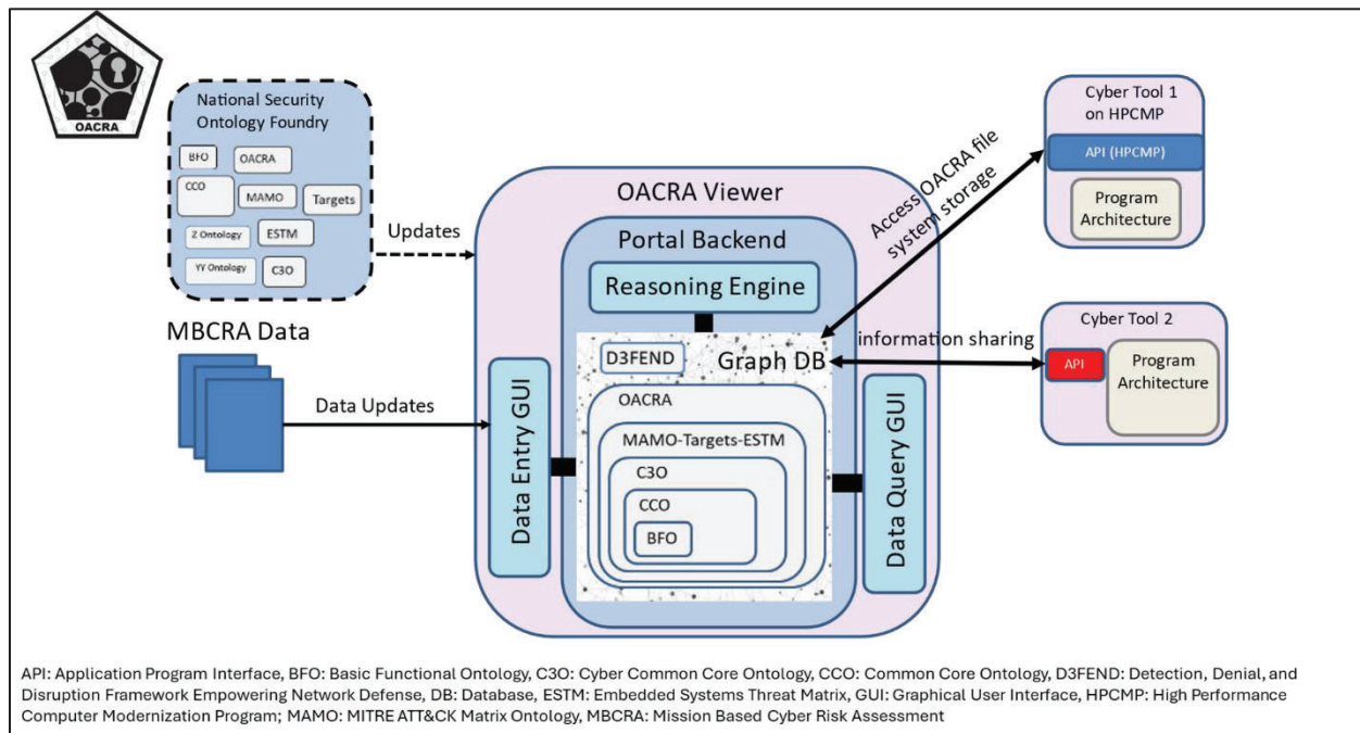
Figure 8-2. The OACRA Viewer Systems View
