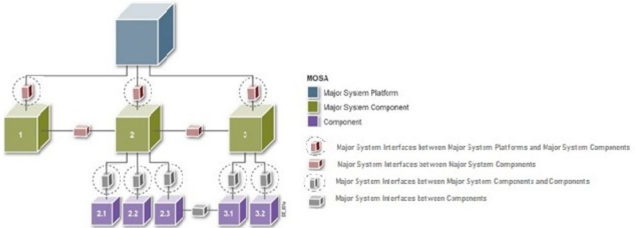
Figure 3-9. MOSA and Modular System Interfaces
