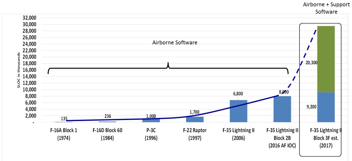
Figure 1. DoD Software Complexity and Growth: Explosive Growth of Source Lines of Code (SLOC) in Avionics Software 3
