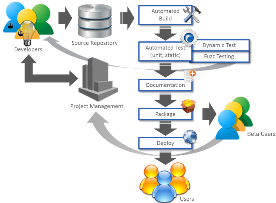
Figure 6. Software Factory
