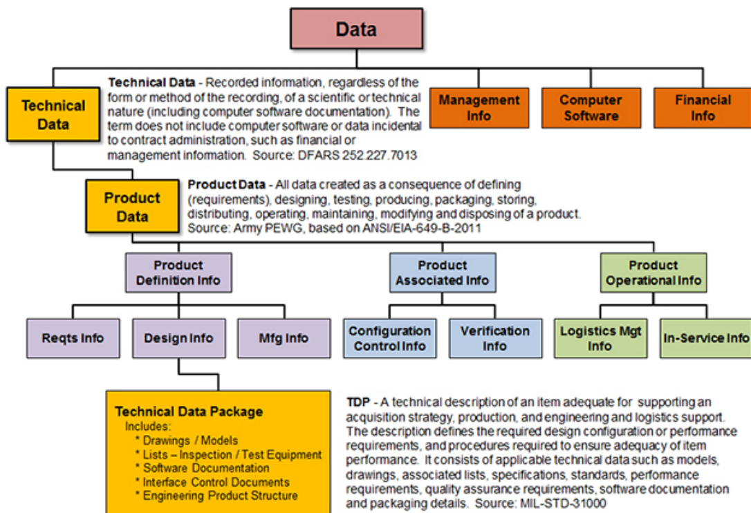
Figure 4-13. Data Taxonomy
