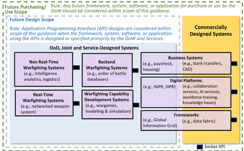
Figure 2. API Design Notional Scope for Future Systems
