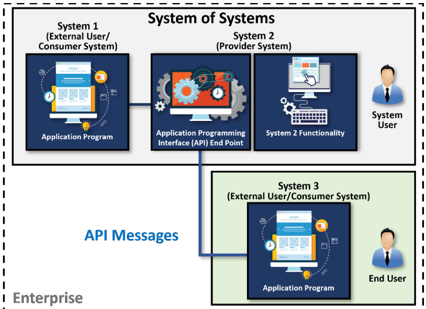
Figure 3. API in a System-of-Systems Context
