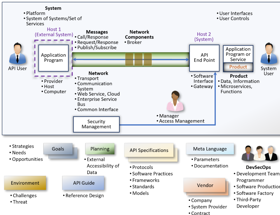
Figure 1. Notional API Ecosystem, Terms, and Relationships
